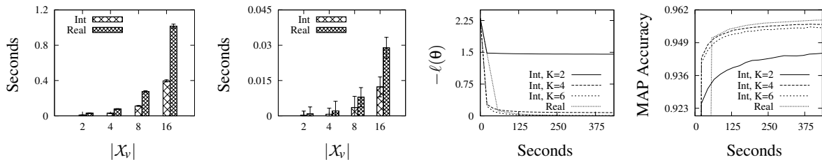
Figure 4: From left to right: Runtime comparison of integer and floating point MRF on two architectures for a varying number of states. (I) Raspberry PI @ 700MHz (ARM11). (II) Intel Core i7-2600K @ 3.4GHz (Sandy Bridge). Progress of stochastic gradient training in terms of (III) training error and (IV) test accuracy as a function of runtime.
