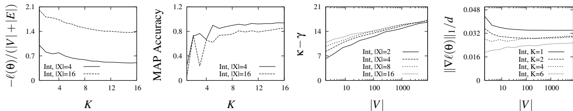
Figure 3: From left to right: (I) negative log-likelihood of IntMRF as a function of K , i.e. the size of the parameter domain. (II) MAP accuracy of MRF as a function of K . (III) Natural size of the parameter domain as a function of the number of vertices (in log-scale) for different state space sizes, whereas \gamma is the smallest and \kappa the largest element of the corresponding estimated parameter vector. (IV) The relative \ell_1 -norm of the gradient for various values of K as a function of the number of vertices (in log-scale).
