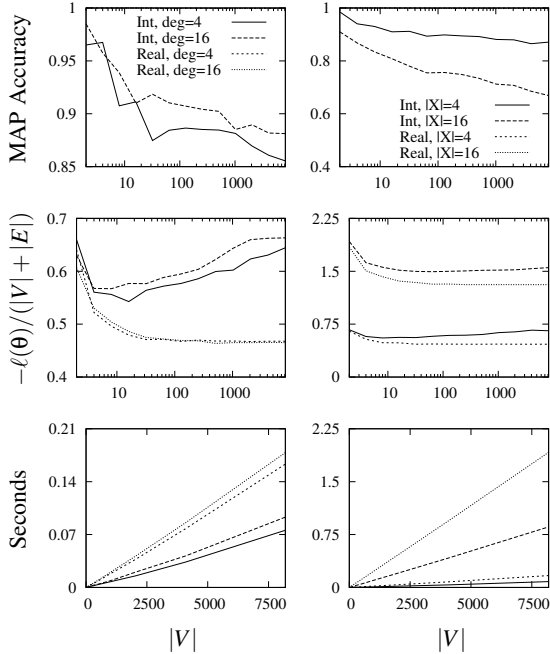
Figure 2: MRF test accuracy (top), training error (center) and runtime in seconds (bottom) for different choices of maximum vertex degree (left column) and state space size (right column) as a function of the number of vertices (x-axis). The plots in each column share the same key that is defined in the top row. The plots in the first two rows have their x-axis in logarithmic scale. IntMRF results are generated with K = 8 .
