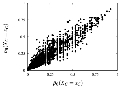
Figure 1: Estimates of edge marginal probabilities for 50 random trees with 50 nodes and 2 states per node. Marginals are computed by the bit length approximation ( \hat{p} ) and vanilla BP ( p ) on the same parameter vector \theta .
